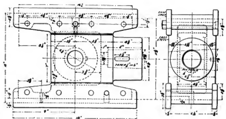
Figs. 1110-1111. Alligator Crosshead.
